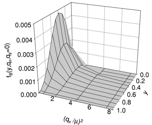
FIG. 6. The boson structure function f_B(y, q_{\perp}) with K=21 , N_{\perp}=7 , \langle:\phi^2(0): \rangle=1 , \Lambda^2=25\mu^2 , and \mu_1^2=10\mu^2 . The transverse momentum is varied with q_y fixed at zero.
