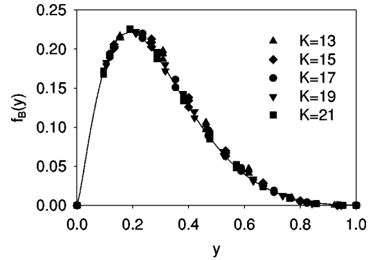
FIG. 11. Same as Fig. 10, but for M^2=10\mu^2 .
