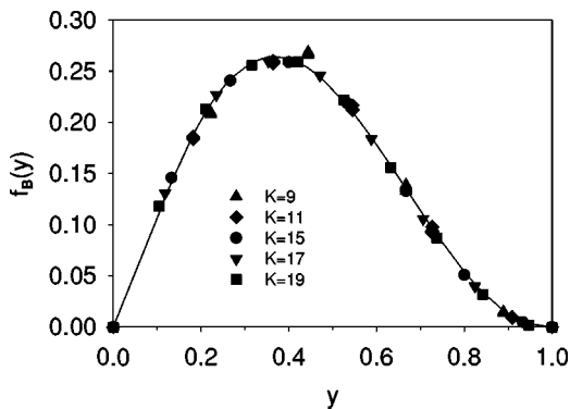
FIG. 1. The boson structure function f_B at various numerical resolutions, with M = \mu , \langle : \phi^2(0) : \rangle = 1 , \Lambda^2 = 50\mu^2 , and \mu_1^2 = 10\mu^2 . The solid line is the parametrized fit, Ay^a(1-y)^b .
