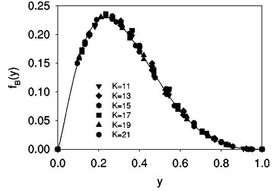
FIG. 10. Same as Fig. 1, but for M^2=5\mu^2 and \Lambda=100\mu^2 and a parametrized fit of Ay^a(1-y)^b e^{-cy} .
