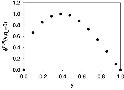
FIG. 3. The boson-fermion two-body amplitude at zero transverse momentum, with K=21 , N_{\perp}=7 , \langle:\phi^2(0): \rangle=1 , \Lambda^2=25\mu^2 , and \mu_1^2=10\mu^2 . The normalization is arbitrary.
