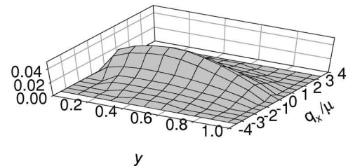
FIG. 2. The one-boson amplitude \phi^{(1,0)} as a function of longitudinal momentum fraction y and one transverse momentum component q_x in the q_y=0 plane. The parameter values are K=21 , N_\perp=7 , \mu_1^2 = 10\mu^2 , \Lambda^2 = 25\mu^2 , and \langle : \phi^2(0) : \rangle = 1 .
