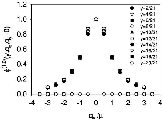
FIG. 4. Cross sections of the boson-fermion two-body amplitude taken at varying longitudinal momenta and at fixed q_y=0 , with K=21 , N_{\perp}=7 , \langle:\phi^2(0): \rangle=1 , \Lambda^2=25\mu^2 , and \mu_1^2=10\mu^2 . The peaks are normalized to be equal at q_x=0 .
