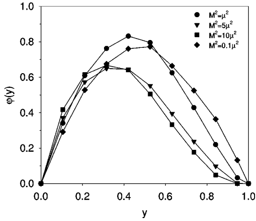
FIG. 13. Comparison of distribution amplitudes \phi(y) \equiv \int d^2 q_\perp \phi^{(1,0)}(y, \mathbf{q}_\perp) for the fermion mass M , with \langle \phi^2(0) \rangle = 1 . The values of the numerical parameters are K=19 , N_\perp=5 , \Lambda^2=50\mu^2 (except for M^2=5\mu^2 and 10\mu^2 when \Lambda^2=100\mu^2 ), and \mu_1^2=10\mu^2 . The lines simply connect the computed points, to guide the eye, and the absolute normalization is arbitrary.
