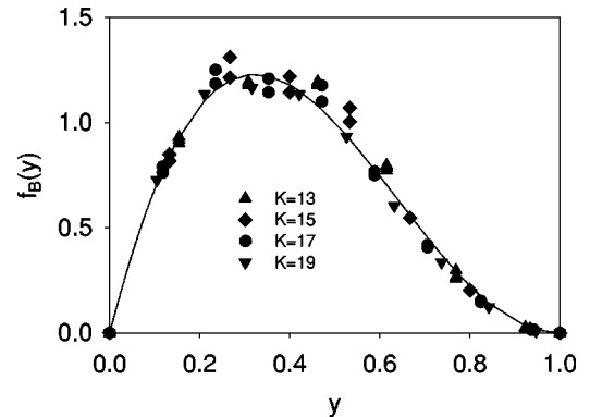
FIG. 12. Same as Fig. 1, but for \langle:\phi^2(0):\rangle=5 .
