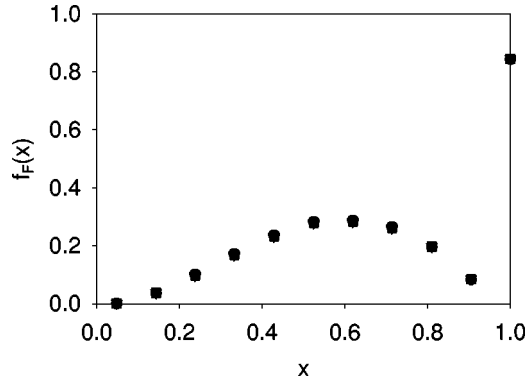
FIG. 7. The fermion structure function f_F with K=21 , N_\perp=5 to 7, \langle:\phi^2(0):\rangle=1 , \Lambda^2=25\mu^2 , and \mu_1^2=10\mu^2 . Each N_\perp value yields essentially the same result.
