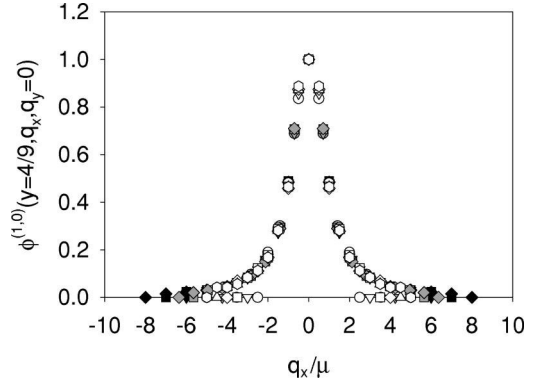
FIG. 5. A cross section of the boson-fermion two-body amplitude taken at fixed longitudinal momentum fraction y=4/9 and at fixed q_y=0 , with K=9 , \langle:\phi^2(0): \rangle=1 , and \mu_1^2=10\mu^2 . The cutoff \Lambda^2 and the transverse resolution N_{\perp} are varied to keep the transverse scale L_{\perp} fixed at one of the following values: 1\pi/\mu (black), \sqrt{2}\pi/\mu (gray), and 2\pi/\mu (white). Different symbol shapes correspond to different values of N_{\perp} . The peaks are normalized to be equal at q_x=0 . The points at zero amplitude mark the transverse range, which is set by the cutoff.
