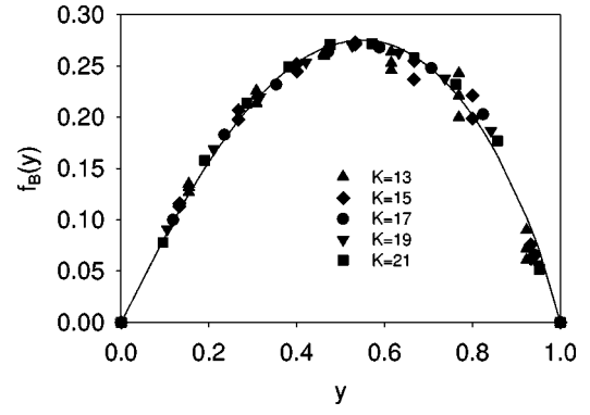
FIG. 9. Same as Fig. 1, but for M^2=0.1\mu^2 .
