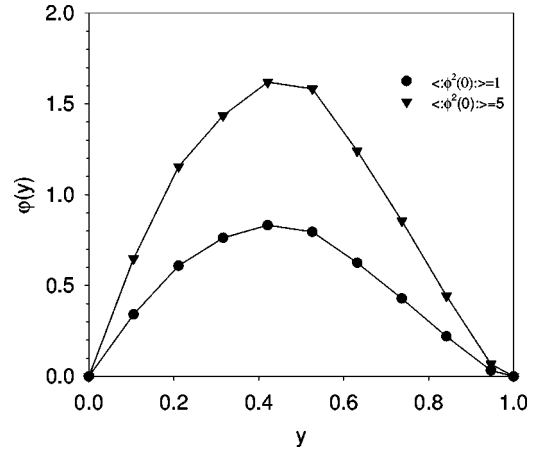
FIG. 14. Same as Fig. 13 but with the fermion mass fixed at M=\mu and \langle \phi^2(0) \rangle varied.
